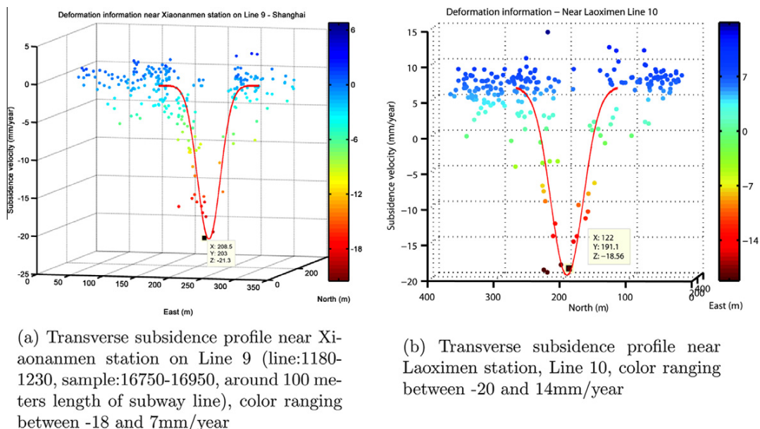
Fig. 9. Subsidence trend profiles of metro lines 9 and 10 in Huangpu District. The vertical axis as well as the color display the settlement velocity in mm/years. The Horizontal axis is expressed in meters in UTM coordinates. (For interpretation of the references to color in this figure legend, the reader is referred to the web version of this article.)
